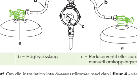
FIGUR 3. STANDARDINSTALLATION - SNABBKOPPLING
